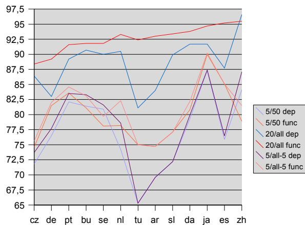
Illustration 2: Performance with different training corpus sizes (upper 2 curves: Ttest data included)
